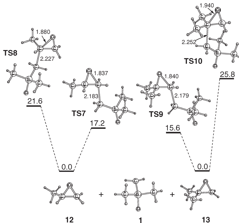
SCHEME 3. Relative Barriers for the Attack of 1 on 2-Methyl-( 12 ) and 2,2-Dimethyloxirane ( 13 ) a
